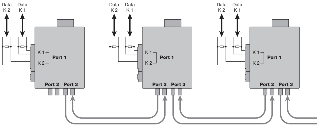
Fig. 3: Half-duplex mode – data channel K1 and data channel K2 are used for data transmission.
