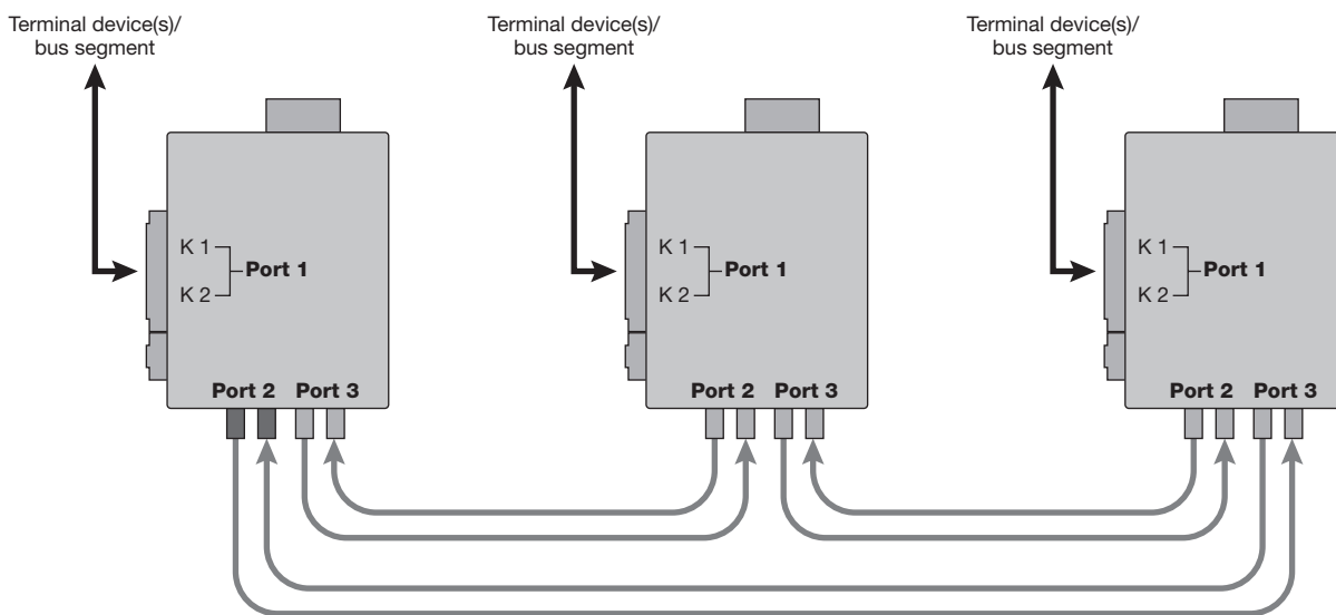
Fig. 9: Redundant ring
