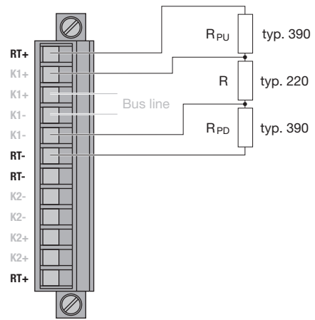
Fig. 17: Termination on the 12-pin screw terminal block for tristate identification through permanent high (terminating resistor and pull-up/pull-down resistors)
