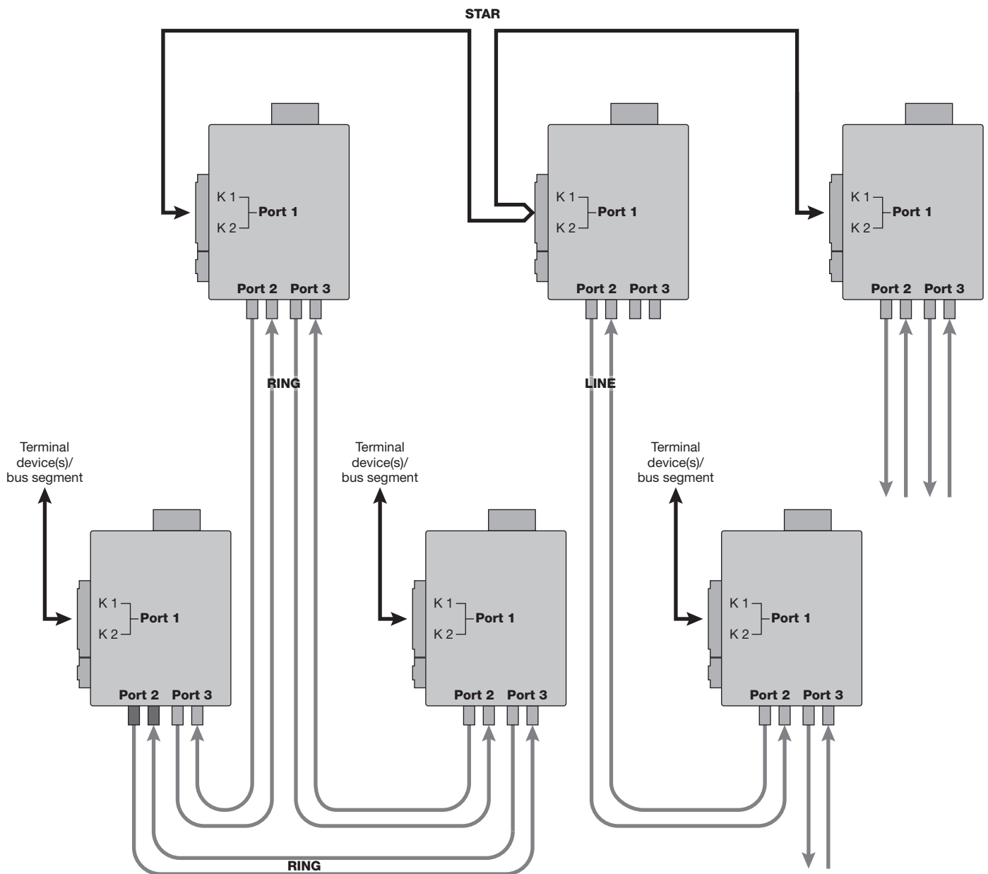
Fig. 10: Star distributor
