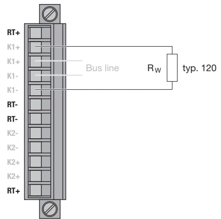
Fig. 18: Termination on the 12-pin screw terminal block for tristate identification through differential voltage (characteristic impedance)
